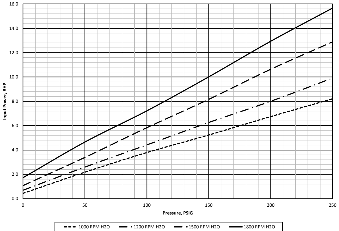
Model CGP80-80 Input Power
