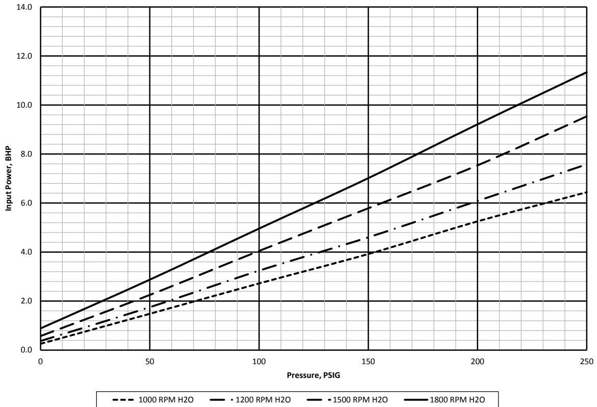
Model CGP80-60 Input Power
