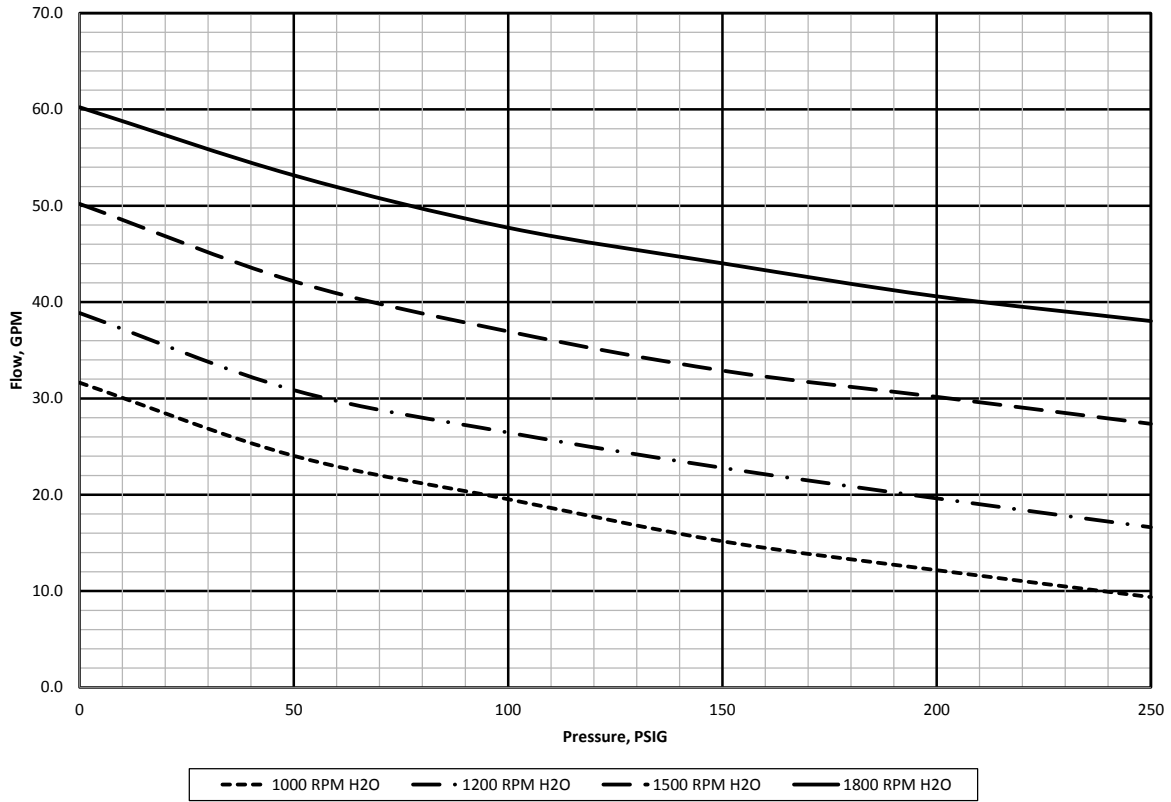
Model CGP80-60 Flow
