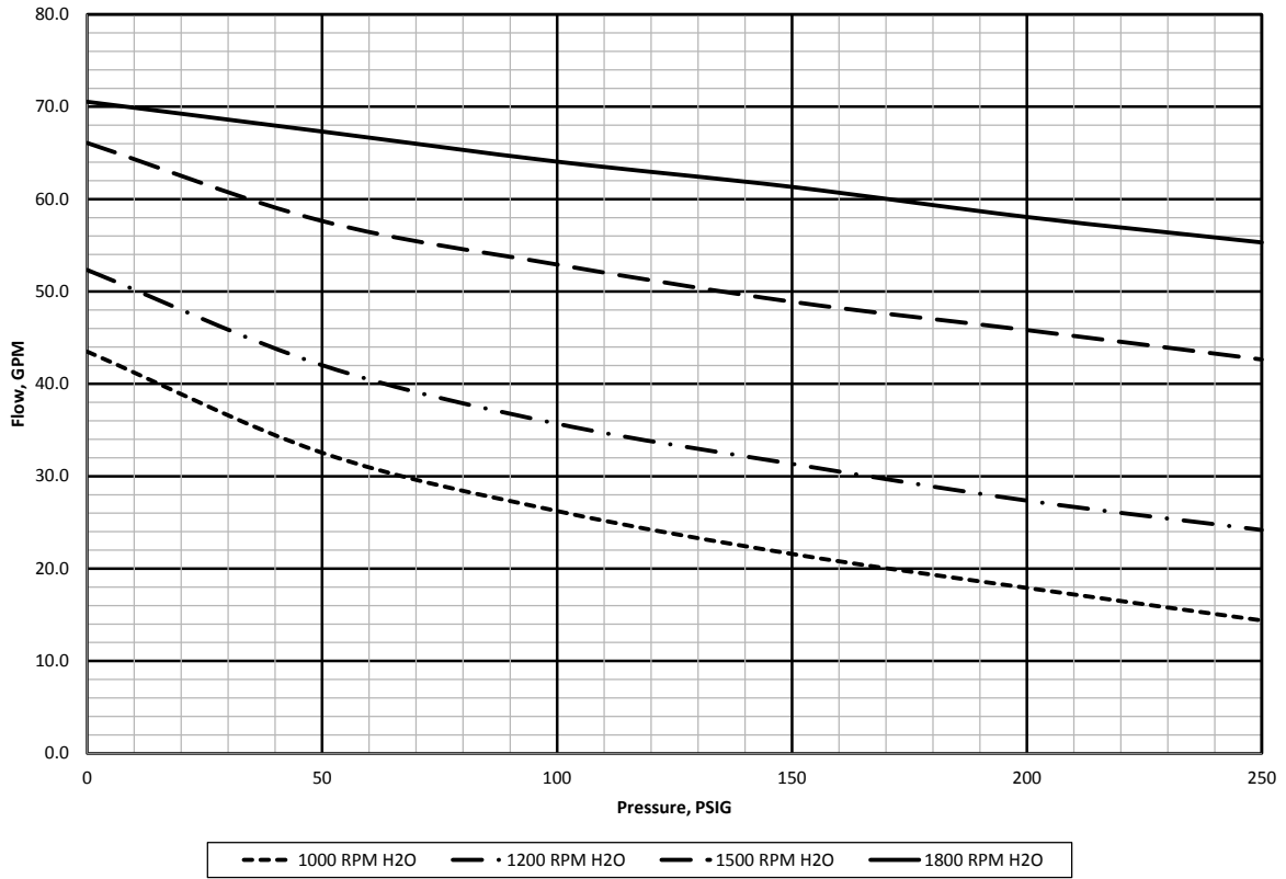
Model CGP80-80 Flow
